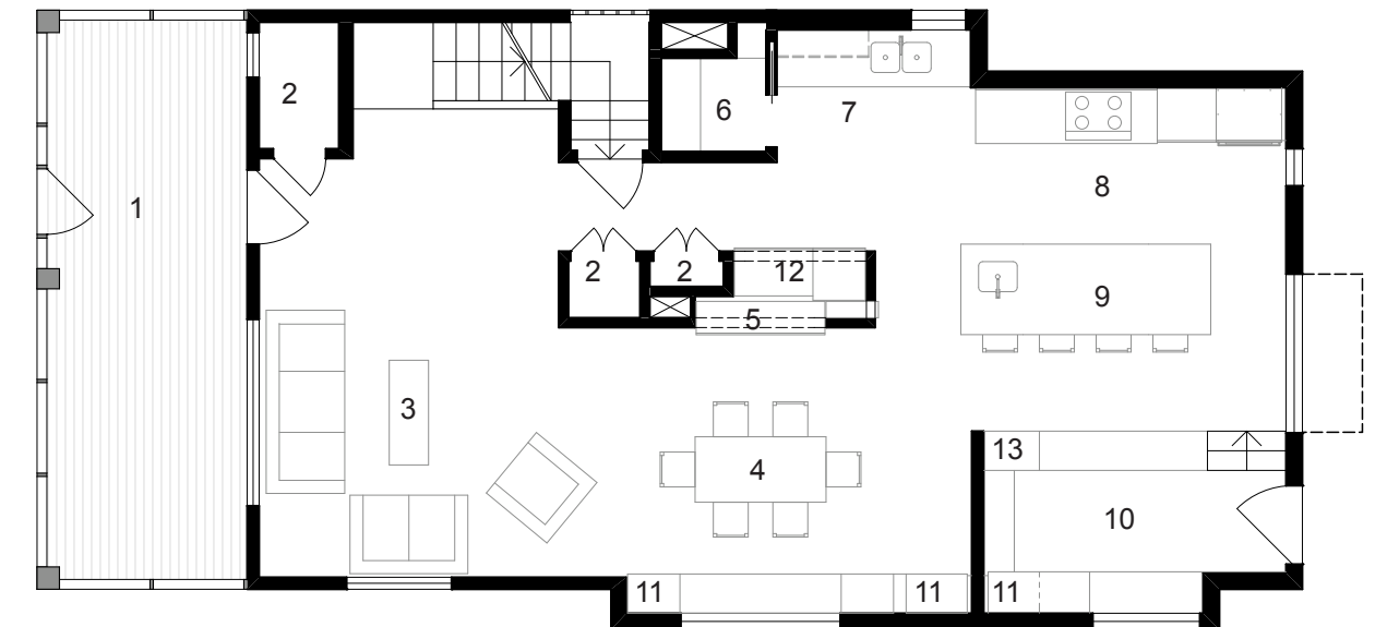
FIRST FLOOR PLAN 1/8" = 1'-0"
