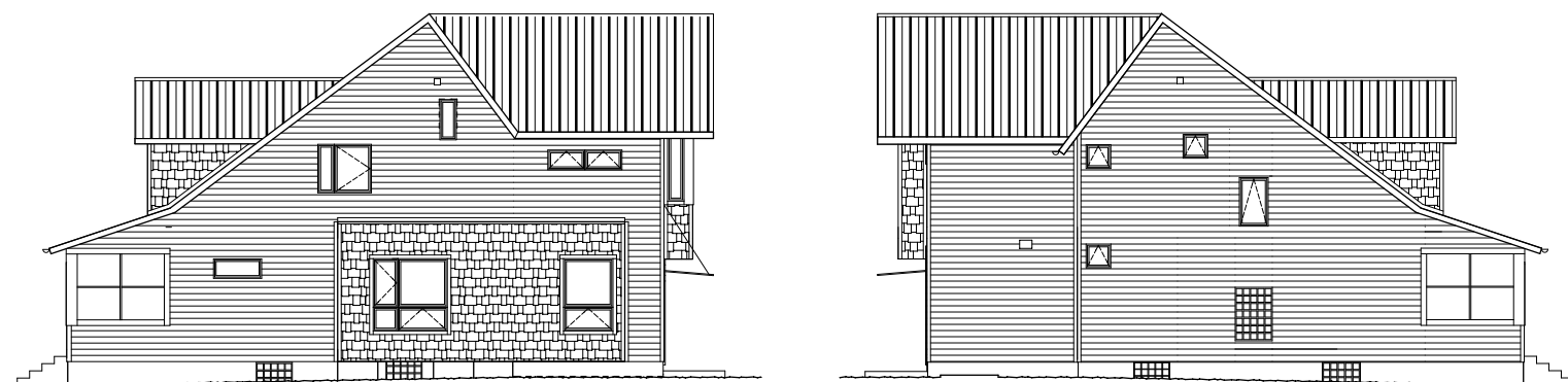
SOUTH & NORTH ELEVATIONS 1/16" = 1'-0"
