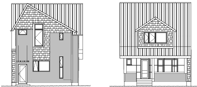
EAST & WEST ELEVATIONS 1/16" = 1'-0"
