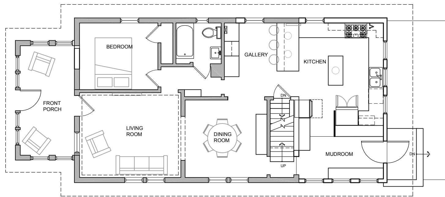
MAIN LEVEL (70% EXISTING, WITH ADDITION)
