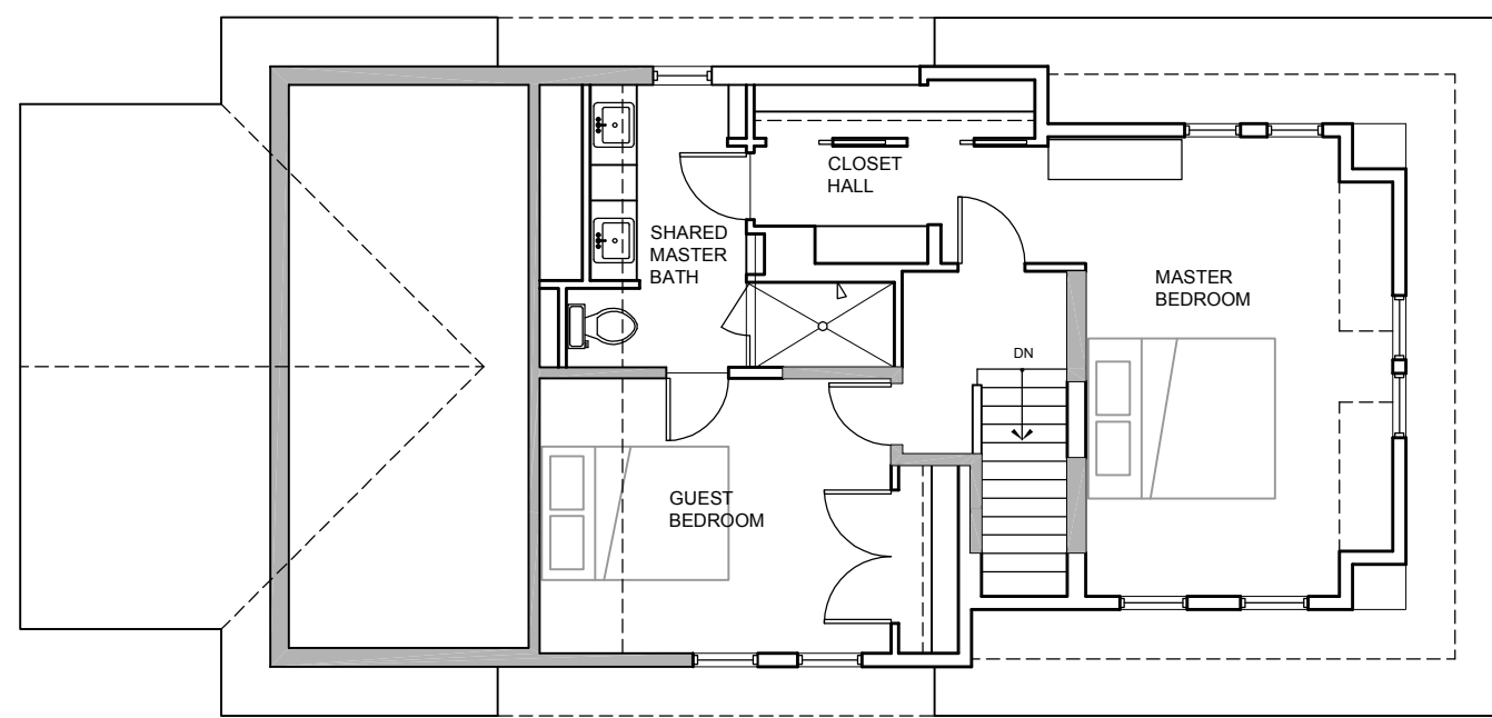
UPPER LEVEL (NEW CONSTRUCTION) 0 2 4 8 16 north
