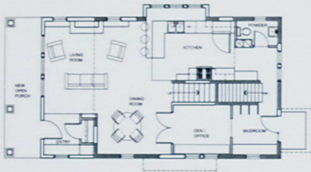
MAIN LEVEL (75% EXISTING, WITH ADDITION)
